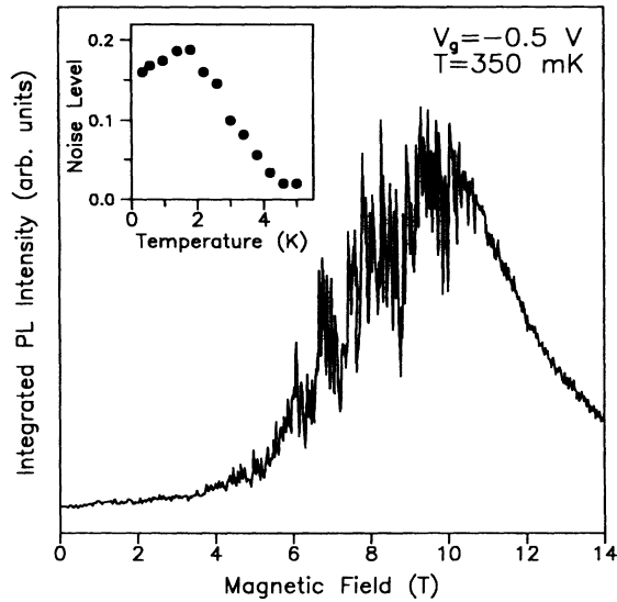
FIG. 4. PL intensity in the indirect regime ( V_g = -0.5 V) at T = 350 mK and ( W_{ex} = -0.5 W/cm 2 ) versus B_{\perp} . Inset: Temperature dependence of the noise level \langle \delta I_{PL} \rangle / \langle I_{PL} \rangle in the indirect regime ( V_g = -0.5 V) at B = 9 T.
