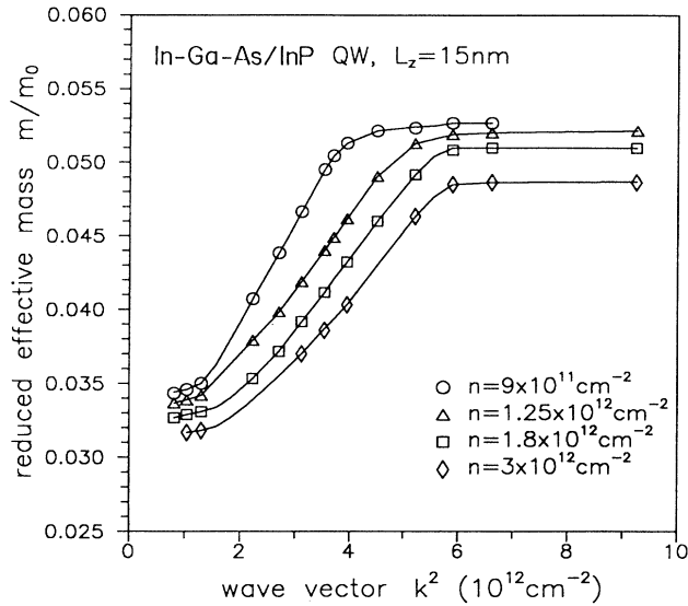
FIG. 10. Dependence of reduced carrier effective mass in a 15-nm QW on square-wave vector for different EHP densities.
