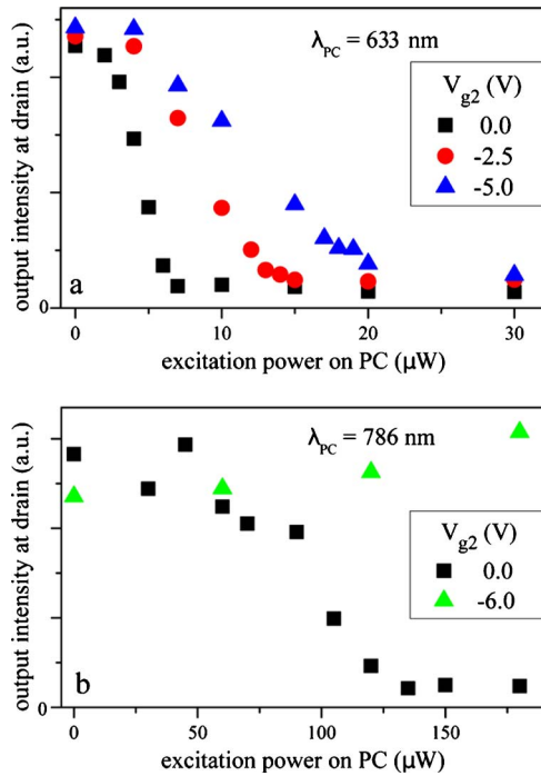
Fig. 3. (Color online) Output intensity integrated over the drain region versus intensity of control light on the PC for different V_{g2} for the control light wavelength, a, \lambda_{PC}=633 and b, 786 nm. In a, V_s=-4.5 , V_d=-5.5 , and V_{g1}=-5.0 V, device a. In b, V_s=-5.5 , V_d=-6.5 , and V_{g1}=-6.0 V, device b.
