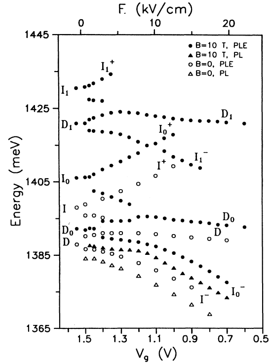
FIG. 4. Electric field dependences of the exciton transition energies at B = 0 and 10 T. PLE line positions at B = 0 ( 10 T) are shown by open circles (solid dots). PL line positions at B = 0 ( 10 T) are shown by open (solid) triangles.
